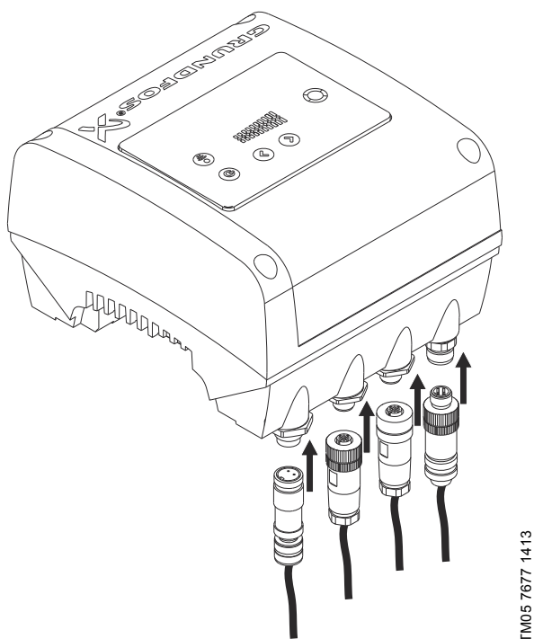
Fig. 41 Fast connection of CME pumps
