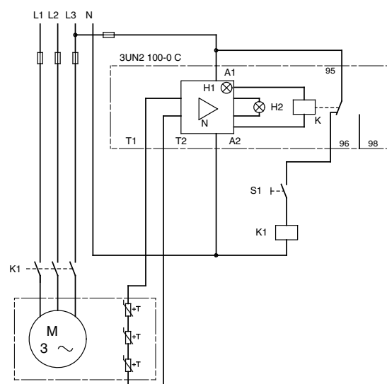
Fig. 45 Three-phase motor with PTC sensors
