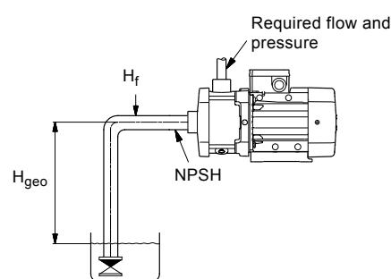
Fig. 30 Dimensional data
